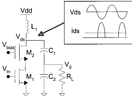
Fig. 6 Schematic of the low-power amplifier
