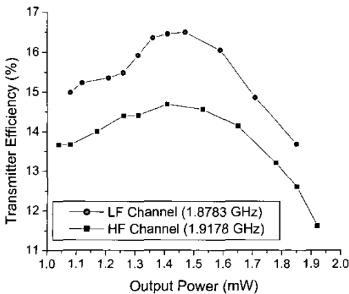
Fig. 12 Transmitter efficiency versus output power
