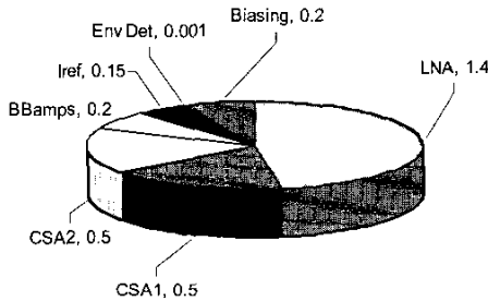
Fig. 11 Receive Current Consumption Breakdown (mA)
