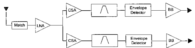
Fig. 1 Receiver Architecture
