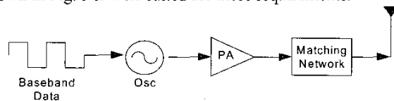
Fig. 5 Direct modulation transmitter architecture
