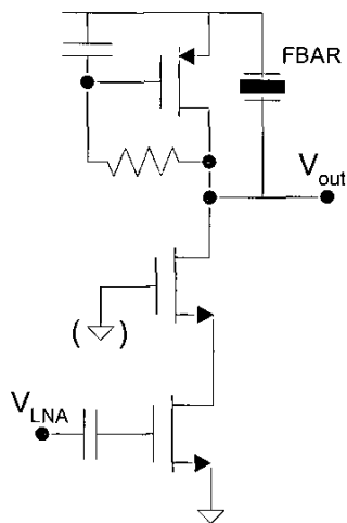
Fig. 3 Channel Select Amplifier Schematic
