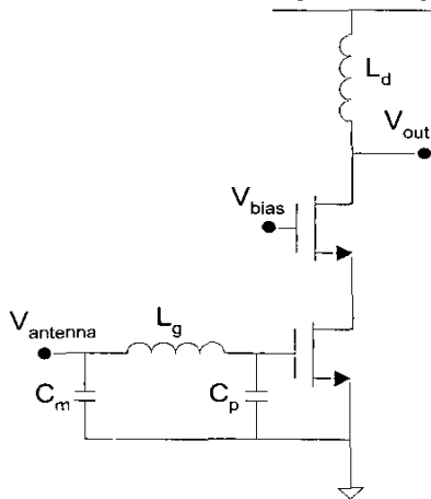
Fig. 2 LNA Schematic
