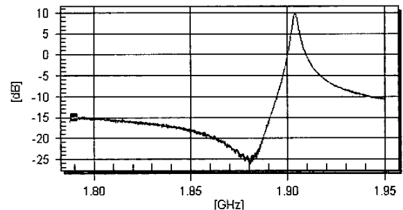
Fig. 8 Measured S21 of Channel Select Amplifier
