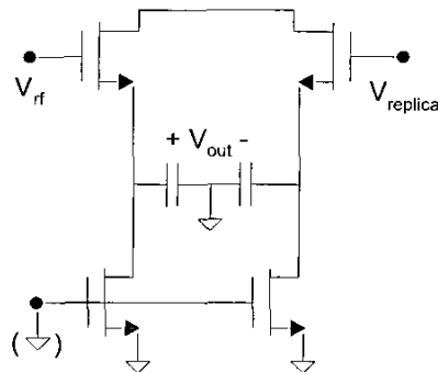
Fig. 4 Envelope Detector Schematic
