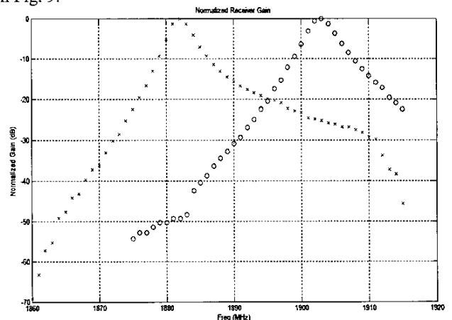
Fig. 9 Normalized Receiver Gain
