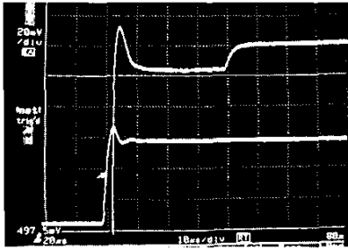
Fig. 10 Receiver Start-Up ( 10\mu\text{s}/\text{div} )
