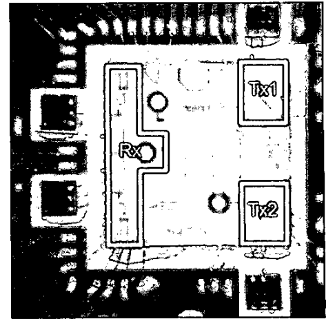
Fig. 7 Transceiver Photograph
